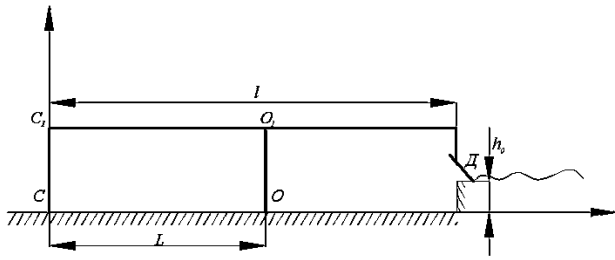
Figure 2 - Model guns feedback with a single push
