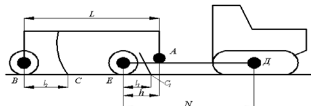
Figure 1 - The structural layout of long-base scheduler
