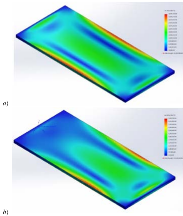
Fig. 4. Stress simulation and the results for the plate with a constant thickness of 8 mm under the uniformly distributed load (a) and the hydrostatic pressure (b) of 24 kPa.
