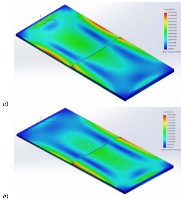
Fig. 5. Stress simulation and the results for the plate with variable thicknesses of 6 mm and 8 mm under the uniformly distributed load (a) and the hydrostatic pressure (b) of 24 kPa
