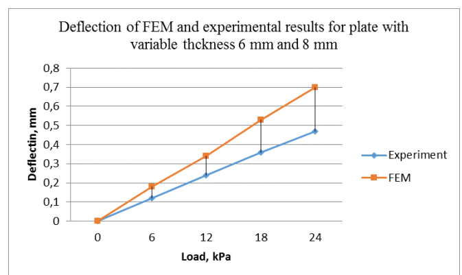
Fig. 7. Deflection for the plate with variable thicknesses of 6 and 8 mm under a distributed load from the experiments and the FEM calculations.
