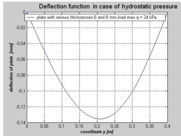
Fig. 3. Curve of deflection for the plate with variable thicknesses of 6 mm and 8 mm loaded by the hydrostatic pressure 24 kPa.
