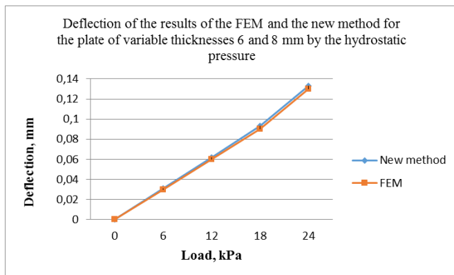
Fig. 9. Deflection for the plate with variable thicknesses of 6 and 8 mm loaded by the hydrostatic pressure from the proposed method and the FEM calculations.
