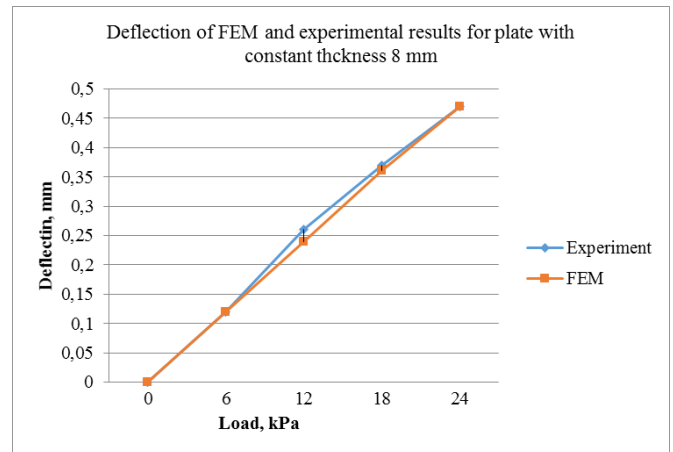
Fig. 6. Deflection for the plate with a constant thickness of 8 mm under uniformly distributed load from the experiments and the FEM calculations.
