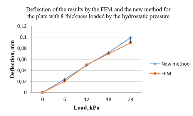
Fig. 8. Deflection for the plate with 8 mm constant thickness loaded by the hydrostatic pressure from the new proposed calculation method and the FEM calculations.
