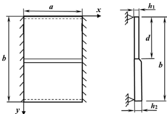
Fig. 2. Rectangular plate with variable thicknesses.
