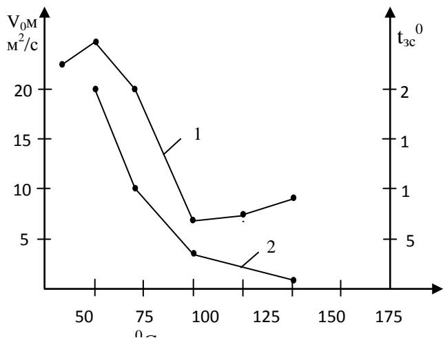
Fig. 1.2. The effect of a temperature of thermal treatment on the rheological parameters of oil 1 – Solidification temperature; 2 – Kinematic viscosity
