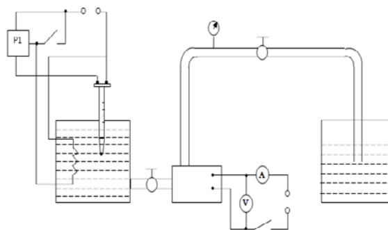
Fig. 1. The principal scheme of the experimental device
