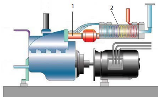
1 - Exhaust gas pipe, 2- Exhaust gas heat exchanger
