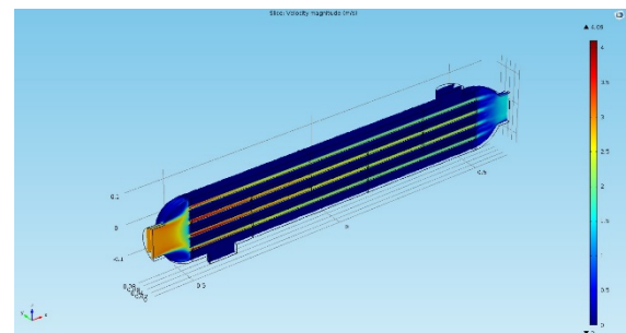
Fig. 12: Simulation of velocity magnitude of exhaust gas heat exchanger in m/s
