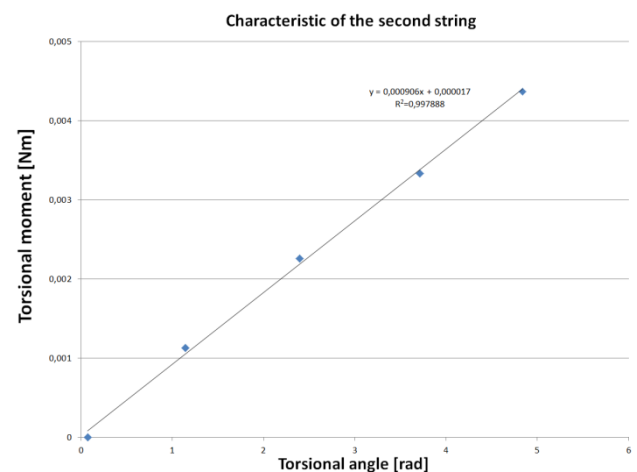
Fig. 8 Characteristic of the second string.
