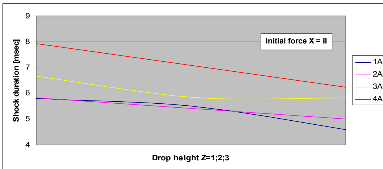
Fig. 9 Impulse duration changing for different programators, angle of drop and initial force II
