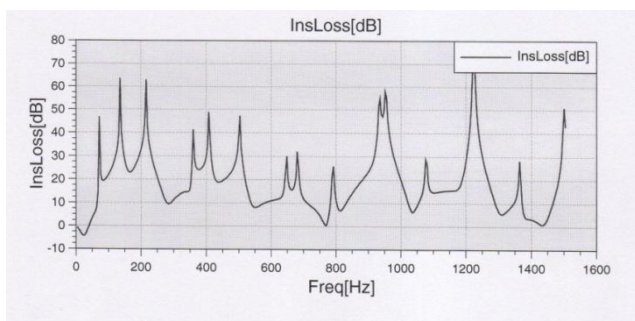
Figure 9. Insertion loss corresponding to configuration of acoustic elements No.3
