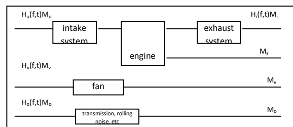
Figure 1. Synergic model of motor vehicle noise generation
